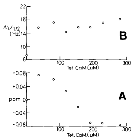
Fig.3. ^{19}\text{F} NMR spectral changes of 0.5 mM TFP ( \text{pH } 7.0 \pm 0.1 ) caused by adding Tet. CaM. (A) Spectral changes in terms of chemical shift in ppm, (B) spectral changes in terms of the half-bandwidth in Hz. The solution consisted of 0.2 M KCl and 2.2 mM \text{CaCl}_2 . Other experimental conditions were the same as in fig.2.
